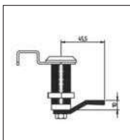
Part no. 21.1093/4
