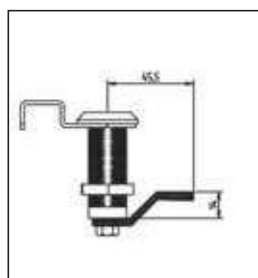
Part no. 21.1093/5
