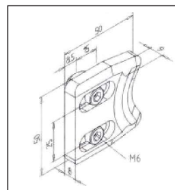
Part no. 21.1767/0
