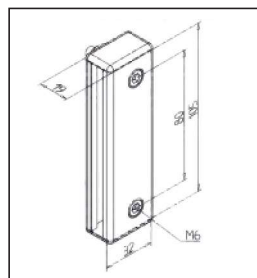
Part no. 21.1755/0
